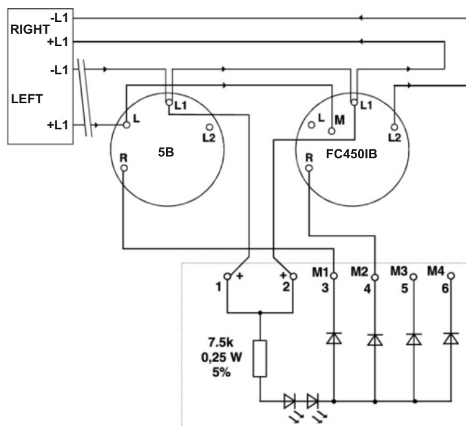
FIG. 2 801HL Simplified Wiring Diagram
